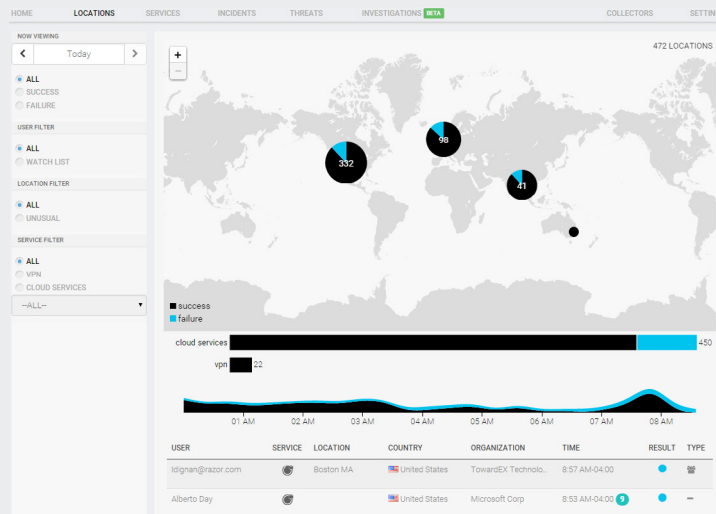
Figure 1: Visualize your organization's cloud authentications
